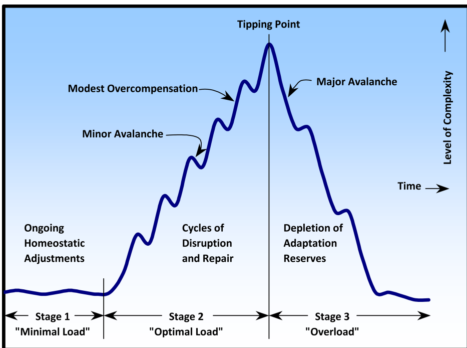
FIGURE 1. Nonlinear evolution of the sandpile over time.
